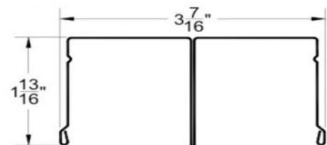
Steel Double Top Track Part # CH21-24
